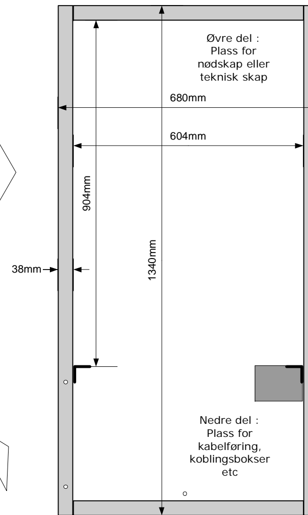
Rack (forfra)
